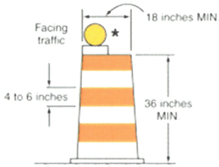
DRUM
