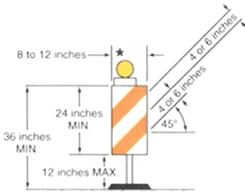
VERTICAL PANEL
